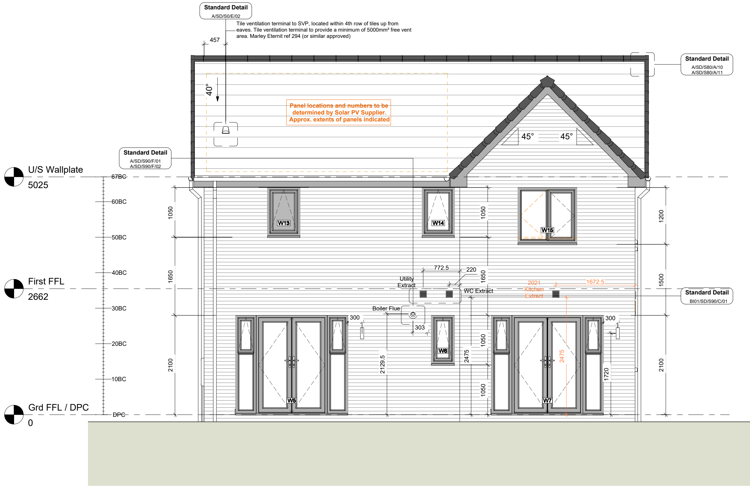
1 Rear Elevation 1 : 50
